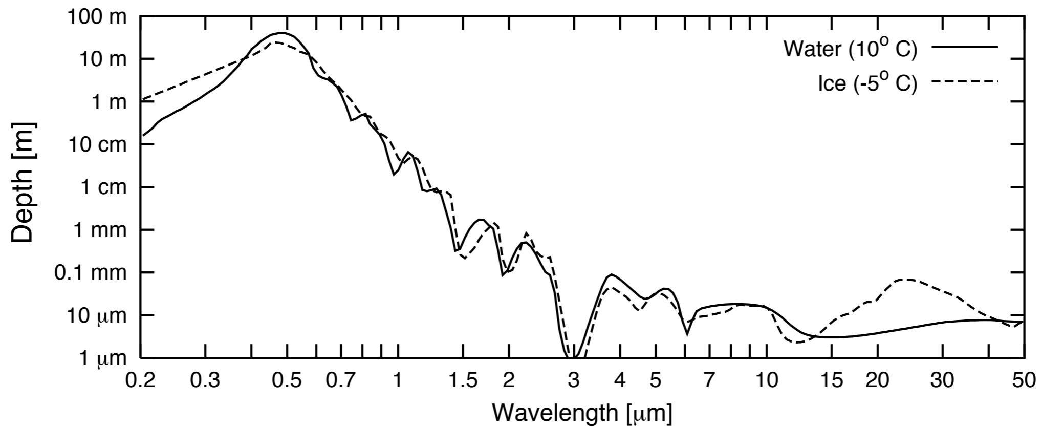
Radiation Penetration Depth in Water and Ice
